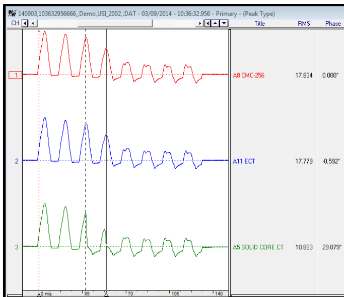
Figure 11: Transformer Inrush Waveform Capture
