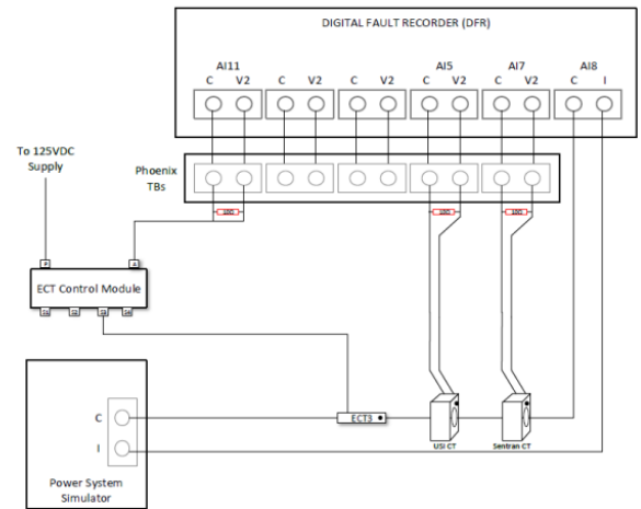
Figure-6: Test setup configuration
