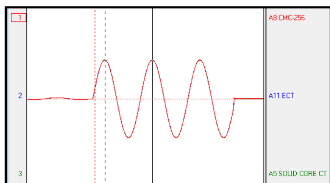
Figure 8: Magnitude and Phase Waveforms Super Imposed
