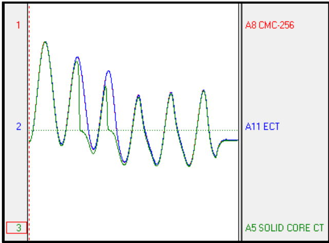
Figure 10: Inrush Waveforms Super Imposed
