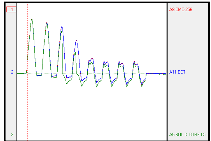
Figure 12: Transformer Inrush Waveforms Super Imposed
