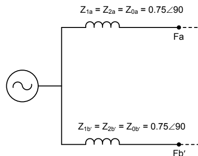
Fig. 26. Simplified impedance diagram
