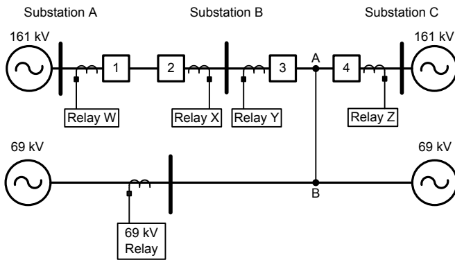
Fig. 18. Intercircuit fault between 161 kV and 69 kV systems
