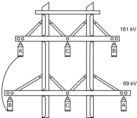
Fig. 19. Tower construction
