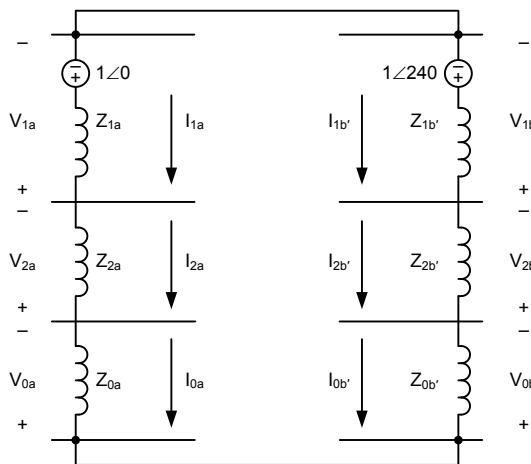
Fig. 24. Thévenin equivalent AB' intercircuit fault
