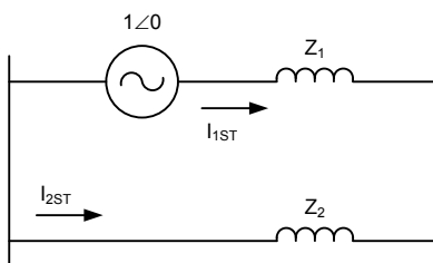
Fig. 28. Sequence diagram for phase-to-phase fault
