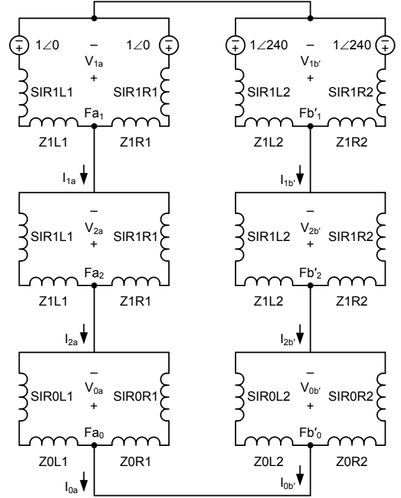
Fig. 23. Total diagram of sequence impedances for AB' intercircuit fault
