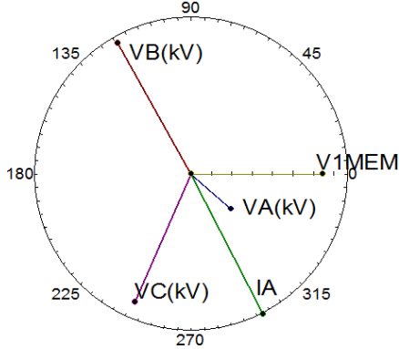
Fig. 9. Phasor diagram of Event #1 from Relay W
