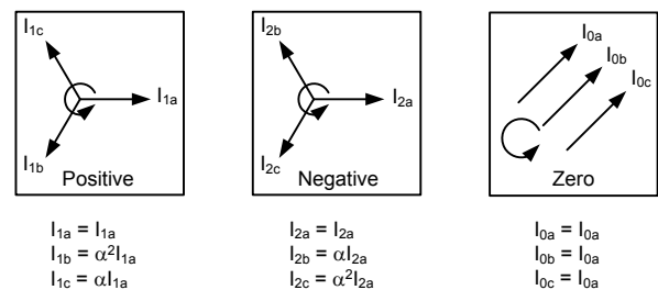
Fig. 20. Phasor relationship for sequence components
