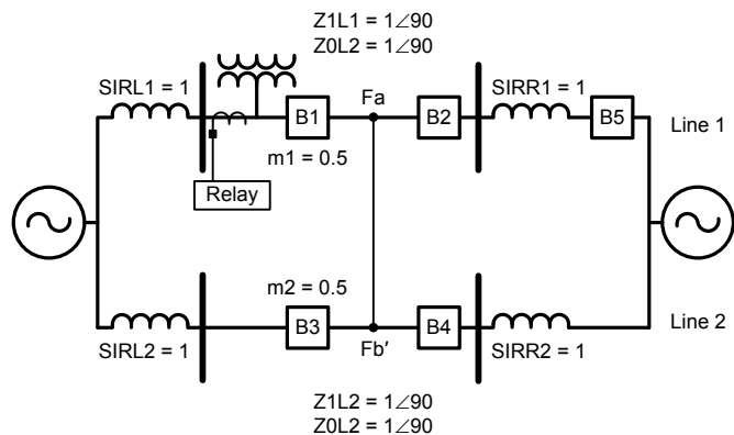
Fig. 25. Example system
