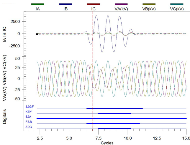
Fig. 14. Event #2 from the 69 kV relay
