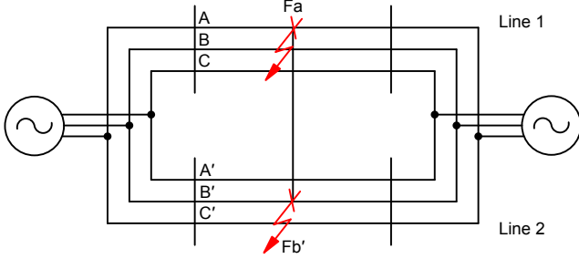
Fig. 21. Basic three-line diagram
