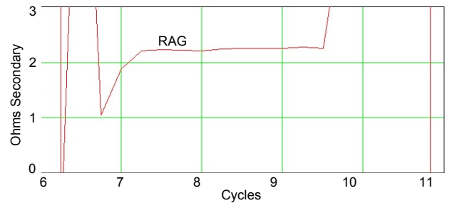
Fig. 8. Fault resistance for Event #1 as calculated by Relay W
