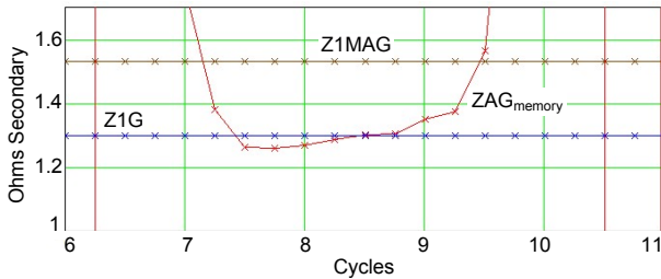
Fig. 6. Ground distance reach evaluation for Event #1 from Relay W
