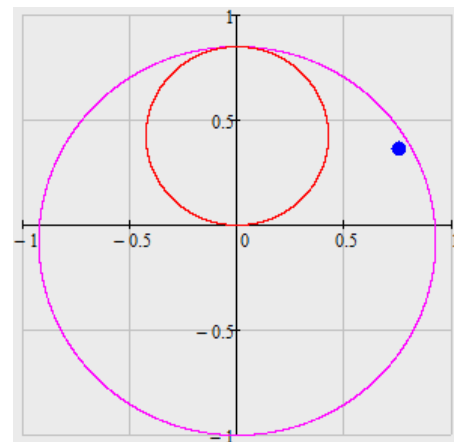
Fig. 32. Memory-polarized mho reach for A-phase-to-ground fault and AB' intercircuit fault at 115 percent of Line 1 with Breaker 5 open
