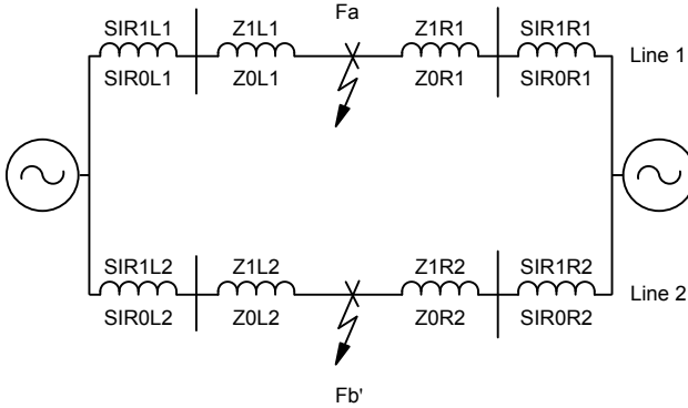
Fig. 22. One-line diagram of system impedances
