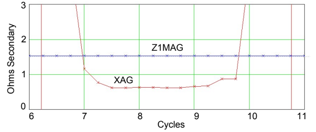
Fig. 7. Calculated line impedance for Event #1 from Relay W
