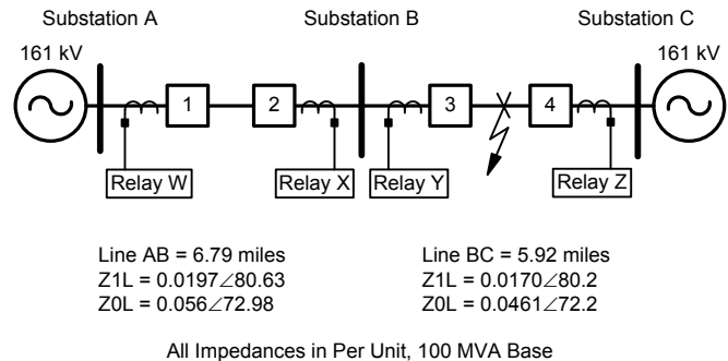
Fig. 1. Simplified one-line diagram of 161 kV system
