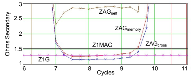
Fig. 10. Distance elements of Event #1 from Relay W
