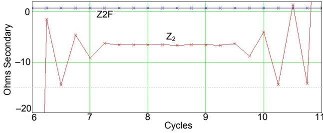
Fig. 5. Z_2 evaluation for Event #1 from Relay W
