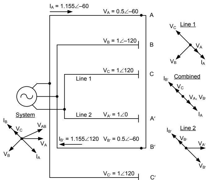
Fig. 27. Fault voltages and fault currents for total system equivalent
