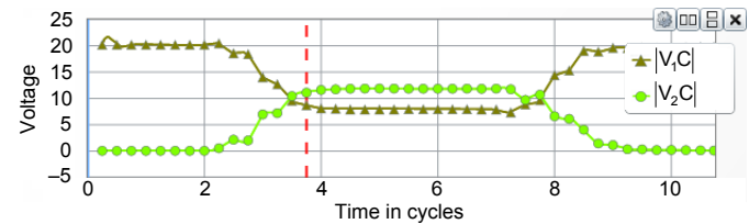
Fig. 15. |V_1C| and |V_2C| for Relay 3
