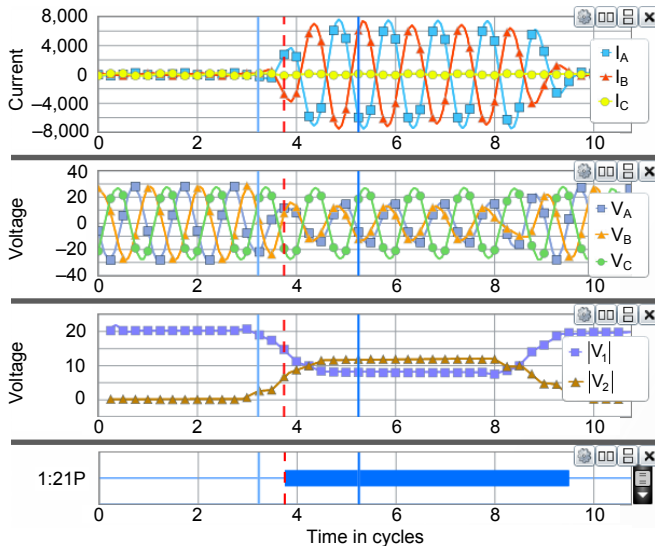
Fig. 8. Relay 2 Event Report Oscillography
