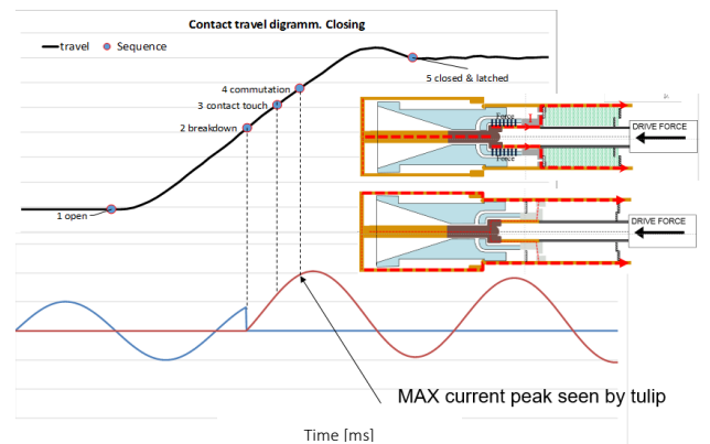
Figure 4 - Current making by closing operation. Travel (black), applied voltage (blue) and current (brown) as function of time. A lower closing speed will increase the time between breakdown and contact touch as well as from contact touch to commutation. This increases the thermal and mechanical stress for the tulip and plug.
