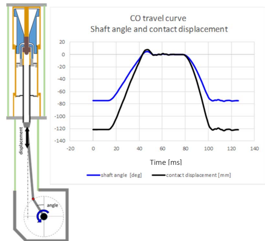
Figure 6 - Example of travel measurement at the bell crank shaft. The relationship between the angle and the displacement is not linear
