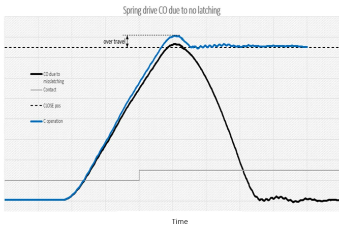
Figure 5 - Travel curve of a circuit breaker with spring operating mechanism. - If the over travel is below the minimum, the latching is not successful and the contacts open again. A Close operation results in a Close-Open sequence.
