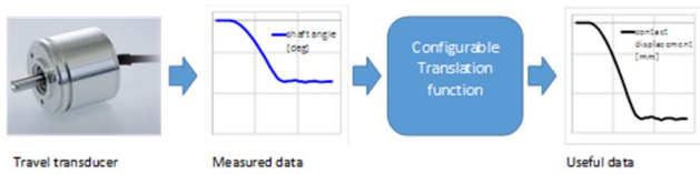
Figure 8 – Principal data processing for getting the actual contact displacement
