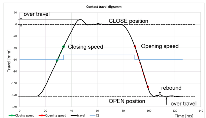
Figure 1 Typical travel curve for a CO operation.
