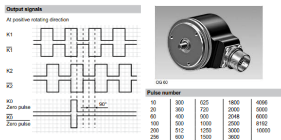
Figure 12. Typical output signal of an incremental encoder. There are two sets of impulses with each set 90 deg shifted from each other that allows determination of the rotational direction. A reference pulse for every revolution (K0) is also given, but not used. The number of pulses per revolution is selectable per the above chart.
