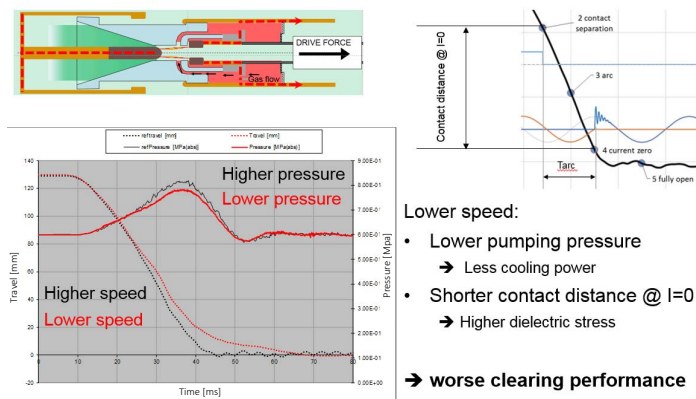
Figure 2- Impact of lower speed on short circuit switching performance. A slower speed results in a smaller mechanical pressure build up in the interrupting chamber. This reduces the blowing pressure at current zero with a consequent reduction of thermal switching capability. Additionally, the contact distance reached for the same arcing time is smaller, which increases the probability of dielectric failure around TRV peak.
