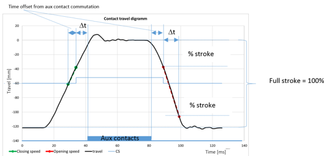
Figure 9 – Travel curve speed evaluation For both opening and closing operation the speed is the average between two points defined independently - 2 for closing - 2 for opening The points can be defined as a % of the total stroke or time.
