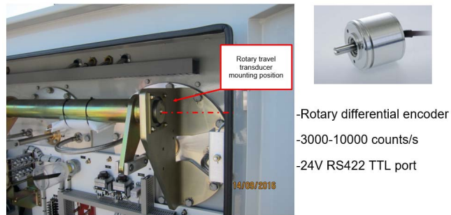
Figure 11 - Rotary transducer
