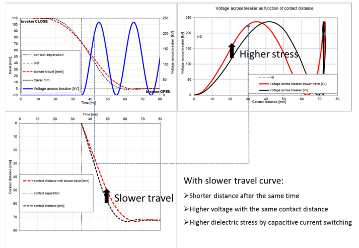
Figure 3 - Capacitive switching.
