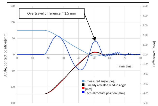
Figure 7 - Travel curve by closing. From the measured angle, linear rescaled measurement and actual contact position are compared. A difference of 1.5 mm could cause 20% to 30% error in the evaluation of the overtravel evaluation.
